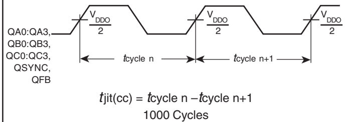
CYCLE-TO-CYCLE JITTER
