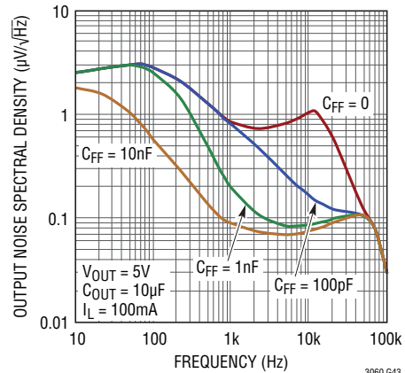
Output Noise Spectral Density vs C_{FF} , C_{REF/BYP} = 10nF
