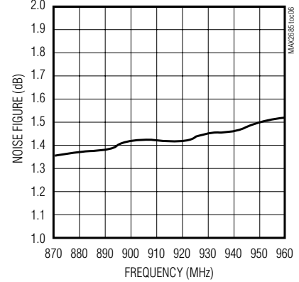
LNA NOISE FIGURE vs. FREQUENCY
