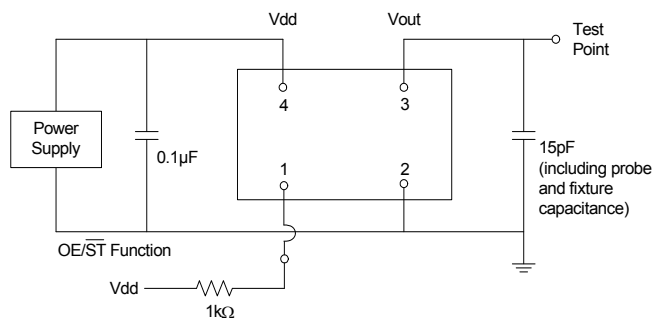
Figure 2. Test Circuit
