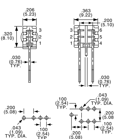
TT21NGVRA1 Vertical Actuation
