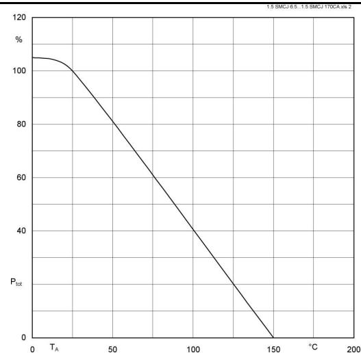
Fig. 2 Rated power dissipation vs. ambient temperature 2)
