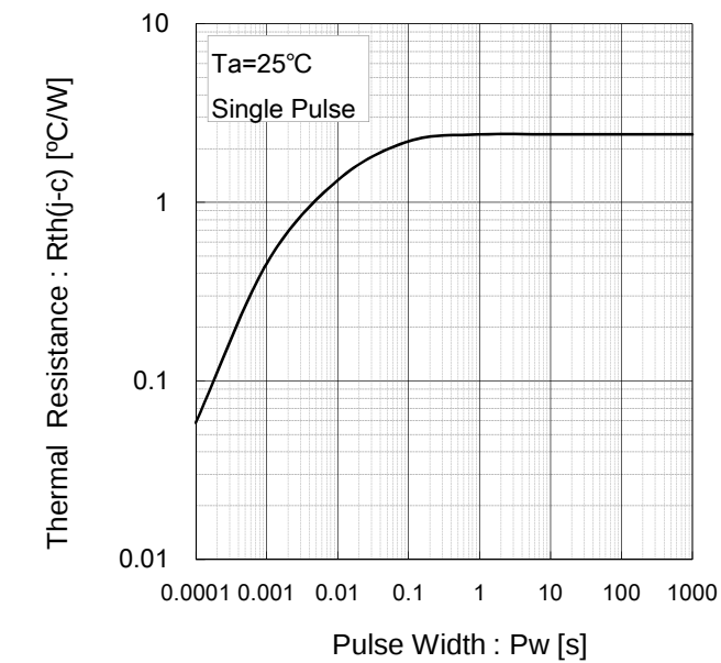
Fig.5 Thermal Resistance vs. Pulse Width
