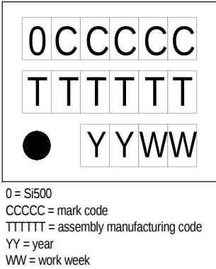
Figure 2. Top Mark
