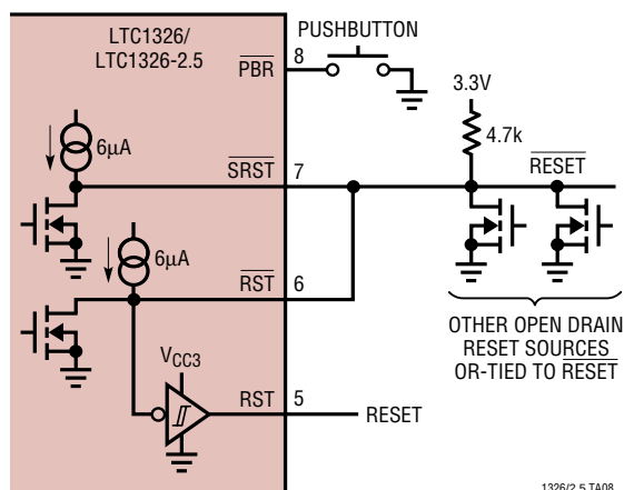
\overline{\text{SRST}} Tied to \overline{\text{RST}} and OR-Tying Other Sources to \overline{\text{RST}} to Generate \overline{\text{Reset}} and \text{Reset}
