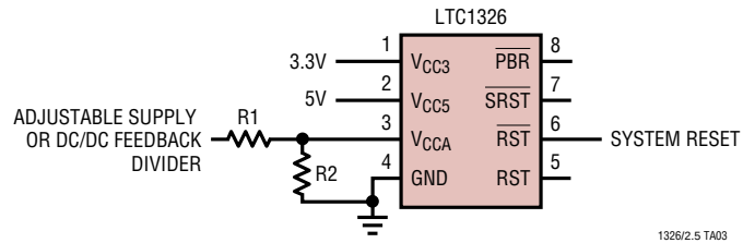
Triple Supply Monitor (3.3V, 5V and Adjustable)
