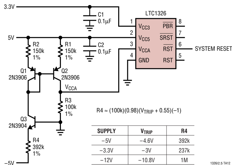
Monitoring a Negative Supply
