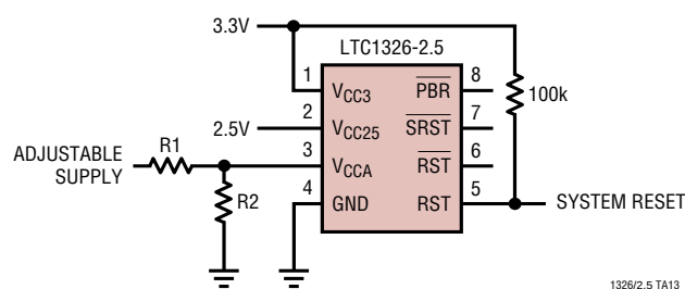
Reset Valid for VCC3 Down to 0V
