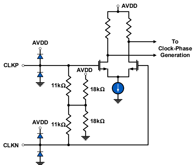
Figure 45. Clock Inputs
