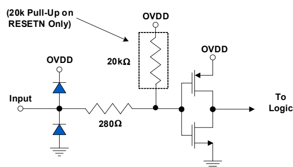
Figure 47. Digital Inputs
