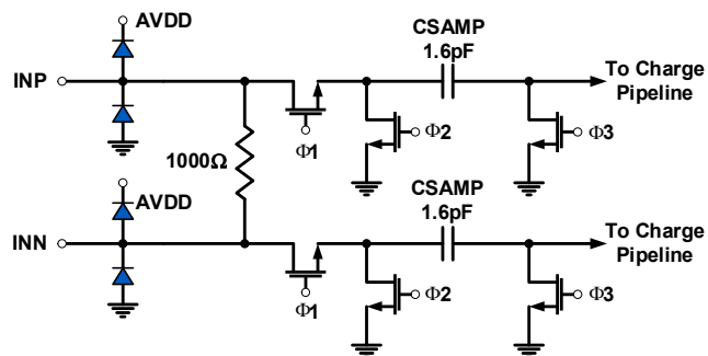
Figure 44. Analog Inputs
