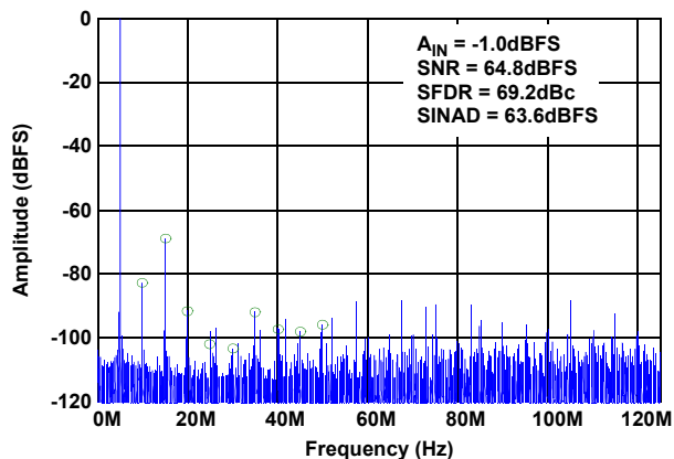
Figure 20. Single-Tone Spectrum at 495MHz
