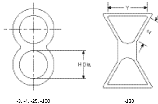
As Supplied (a)
