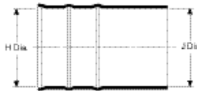
After Unrestricted Recovery (b)
