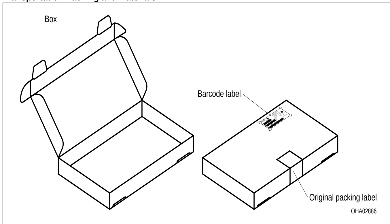
Dimensions of transportation box in mm (inch)
