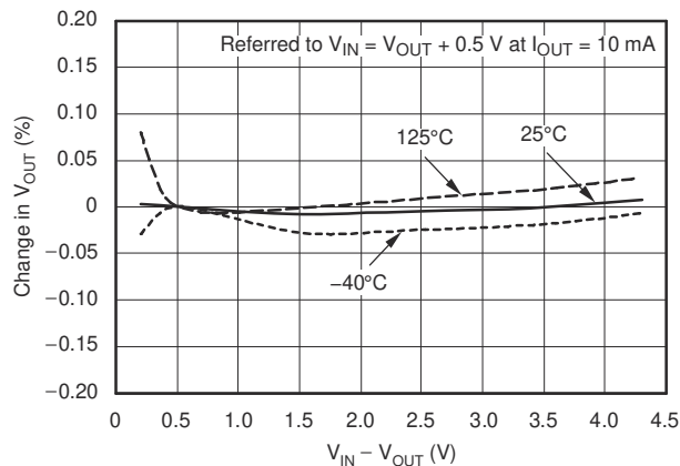
Figure 5-2. Line Regulation
