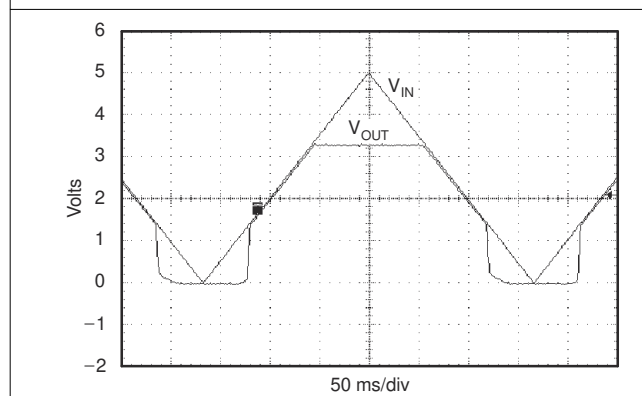
Figure 5-21. TPS73633 Turn-On Response
