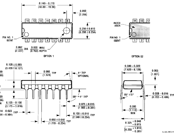
14-Lead Molded Dual-In-Line Package (N) Order Number DM74LS15N NS Package Number N14A
