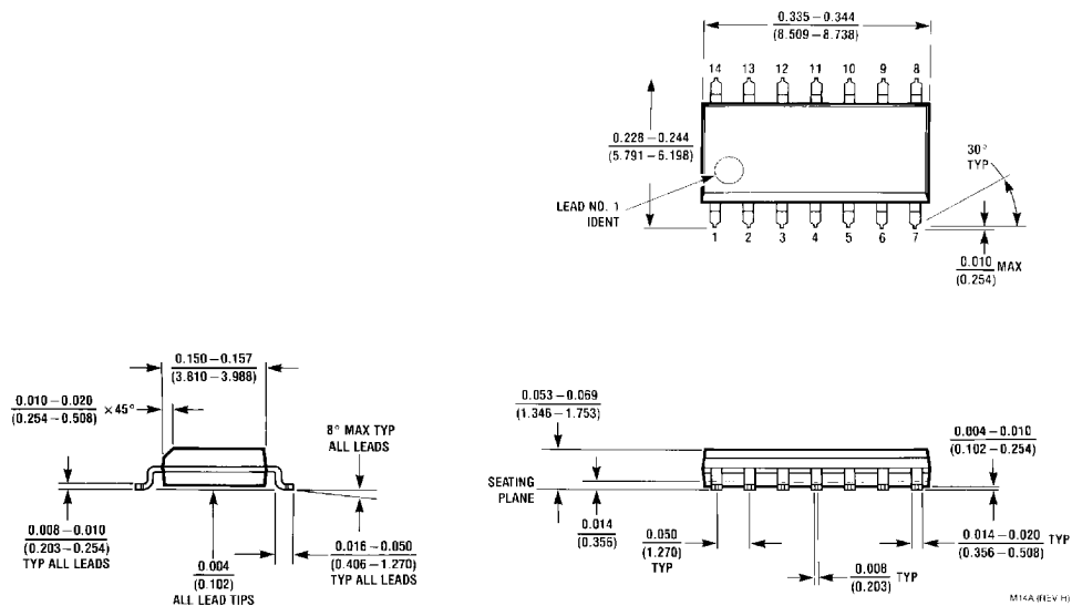
14-Lead Small Outline Molded Package (M) Order Number DM74LS15M NS Package Number M14A
