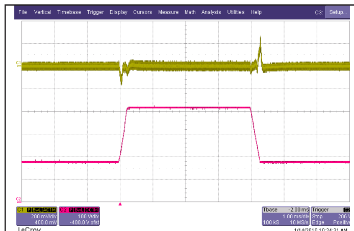
Figure 6: Output voltage response to step-change in input voltage (180V - 425V - 180V), at 50A load current. Load cap: 15μF tantalum capacitor and 1μF ceramic cap. Ch 1: V out (200mV/div), Ch 2: V in (100V/div).
