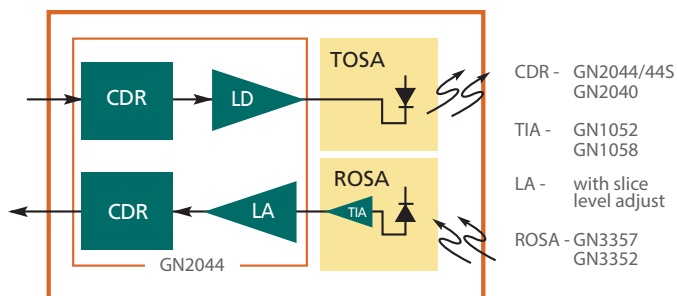
10G XFP Module for \leq 80 Km Applications
