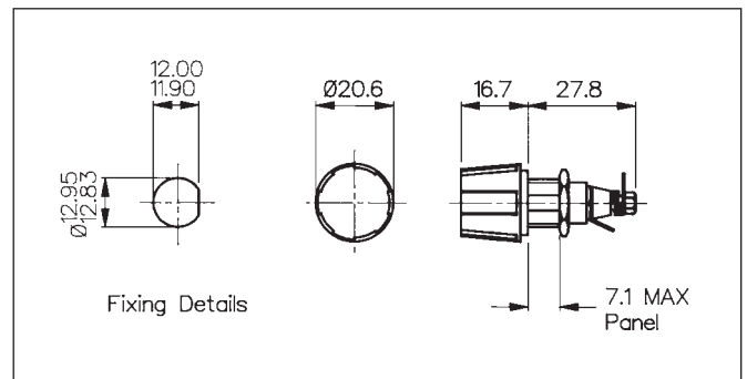
Fixing Details
