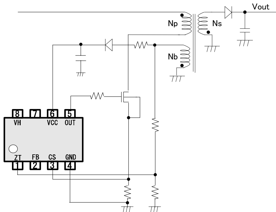
Fig-12 How to Set VCCOVP
