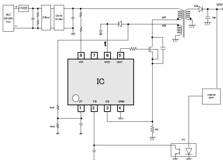
Fig 1. Application Circuit
