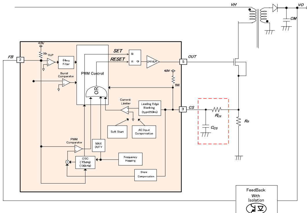
Fig-17. CS pin surrounding circuit
