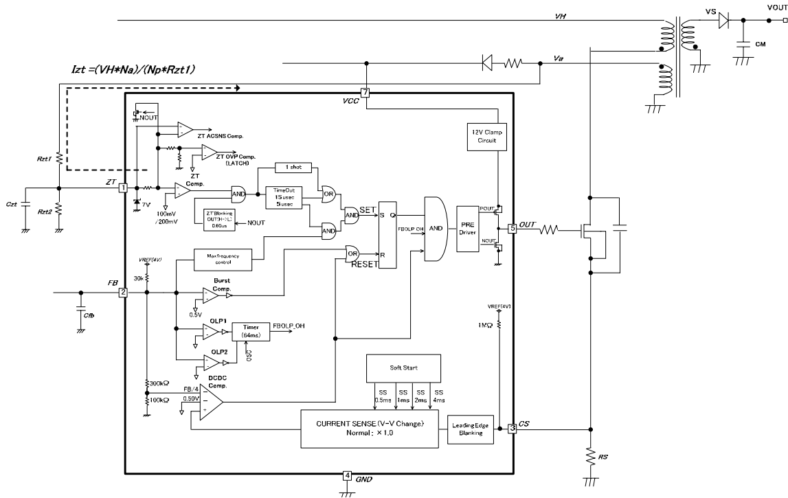
Fig-14 DC/DC Operation Block
