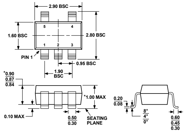
Figure 37. 5-Lead Thin Small Outline Transistor Package [TSOT] (UJ-5) Dimensions shown in millimeters
