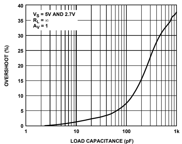
Figure 20. Small Signal Overshoot vs. Load Capacitance
