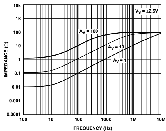
Figure 19. Closed-Loop Output Impedance vs. Frequency
