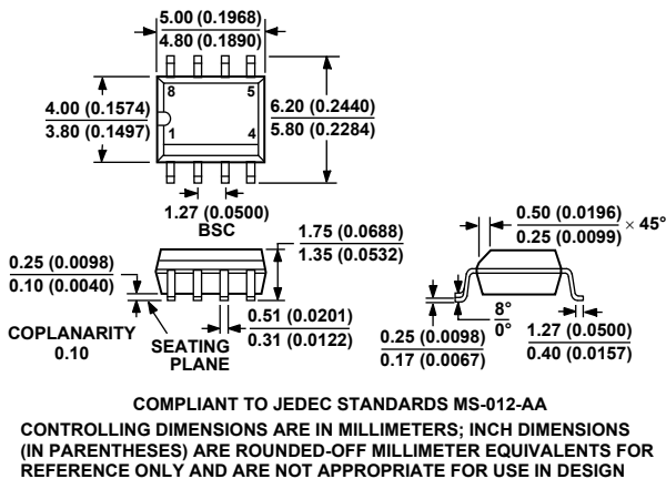
Figure 36. 8-Lead Standard Small Outline Package [SOIC] Narrow Body (R-8) Dimensions shown in millimeters and (inches)
