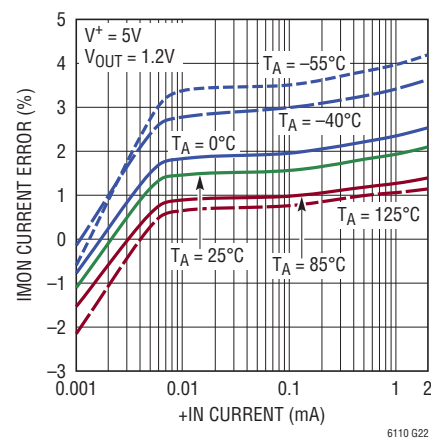
IMON Current Error vs +IN Current
