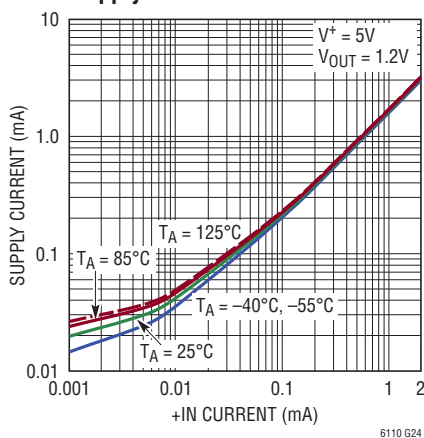
Supply Current vs +IN Current
