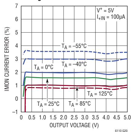
IMON Current Error vs Output Voltage
