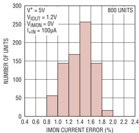
IMON Current Error Distribution
