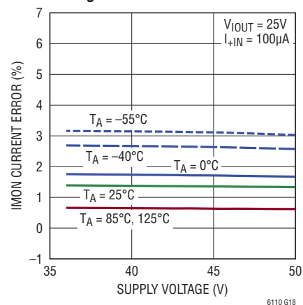
IMON Current Error vs Supply Voltage
