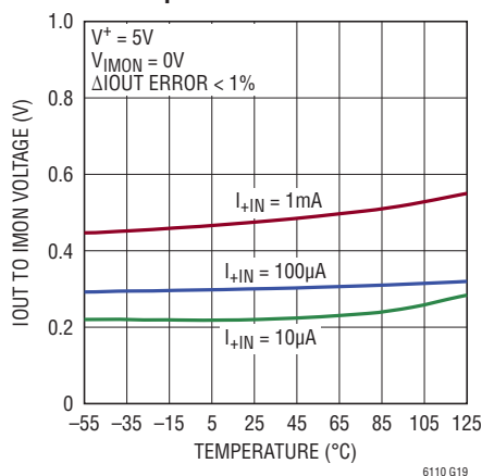
Minimum IOUT to IMON Voltage vs Temperature
