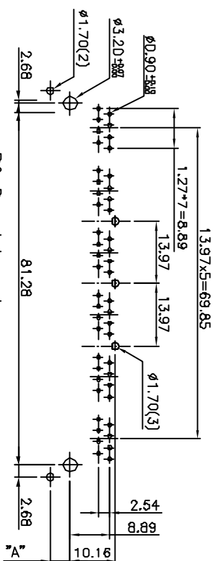
PC Board Layout
