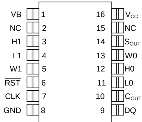
16-Pin SO (300-mil) See Mech. Drawings Section
