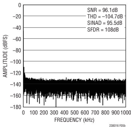
Figure 5b. 32k Point FFT Plot with f_{IN} = 2kHz for Circuit Shown in Figure 5a
