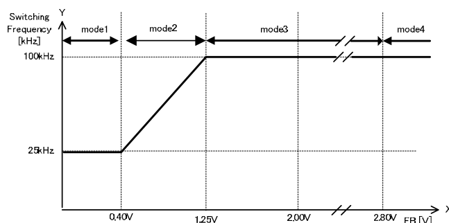
Figure-11-2. Switching operation state (BM1P10x series)
