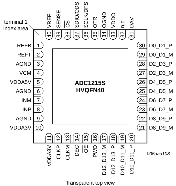
Fig 3. Pin configuration with LVDS/DDR digital outputs selected
