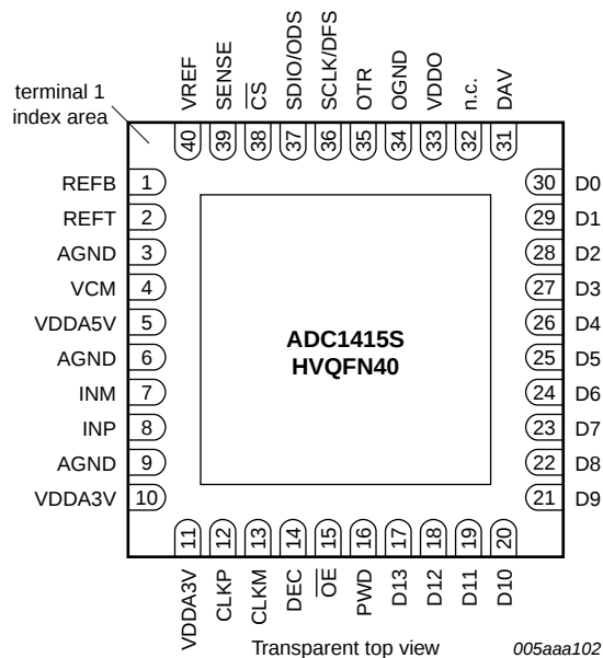
Fig 2. Pin configuration with CMOS digital outputs selected
