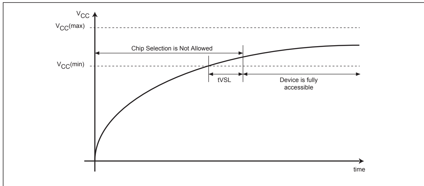
Figure 29. Power-up Timing
