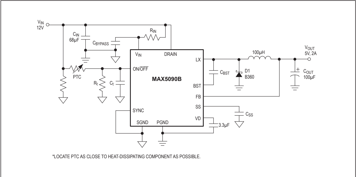
Figure 5. Load-Temperature Monitoring with ON/OFF (Requires Accurate V_{IN} )
