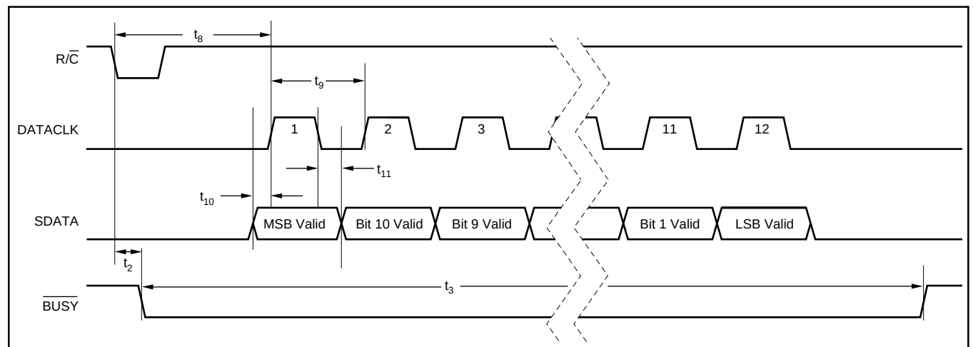
FIGURE 2. Serial Data Timing Using Internal Clock. ( \overline{CS} , EXT/ \overline{INT} and TAG Tied LOW.)
