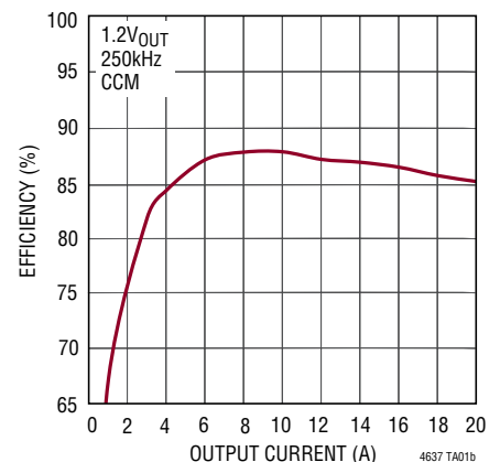
12V IN Efficiency vs Load Current
