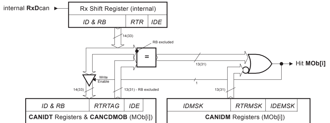
Figure 16-10. Acceptance Filter Block Diagram
