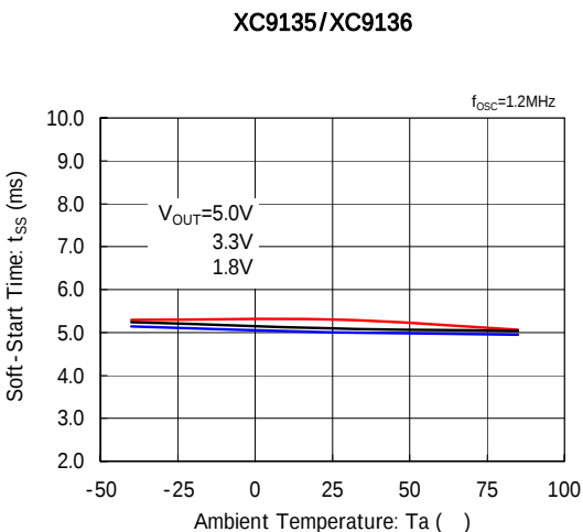
(12) Soft-Start Time vs. Ambient Temperature
