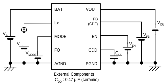
< Circuit No.4 >
