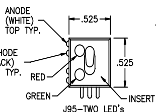
J95—TWO LED's
