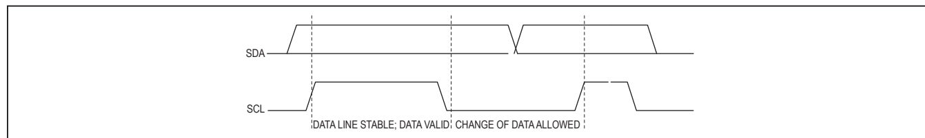
Figure 4. Bit Transfer
