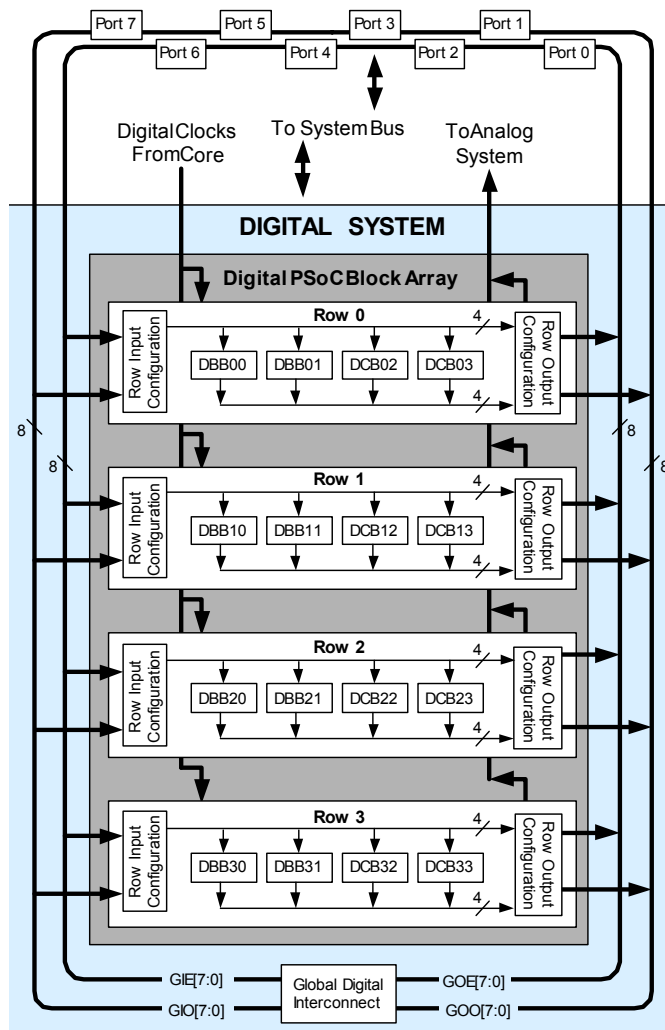
Figure 3-3. Digital System Block Diagram
