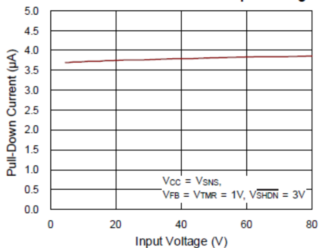
TMR Pull-Down Current vs. Input Voltage
