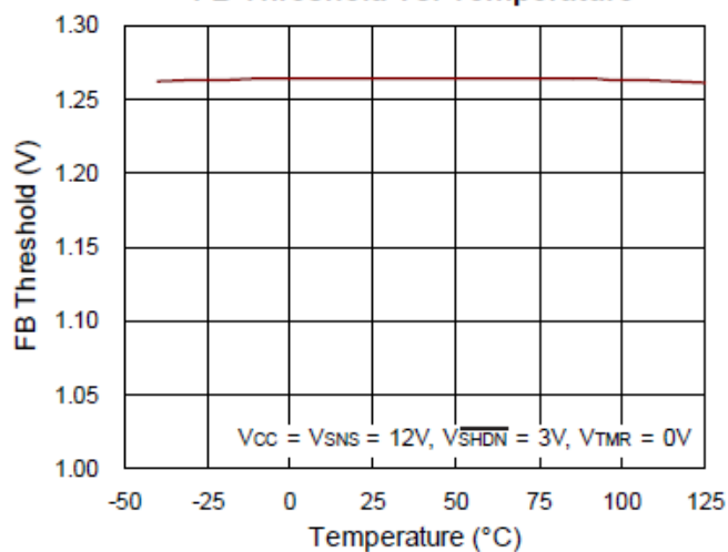
FB Threshold vs. Temperature
