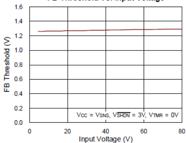
FB Threshold vs. Input Voltage
