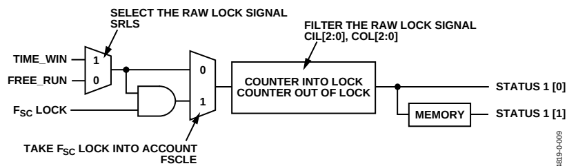
Figure 8. SDP Lock Related Signal Path
