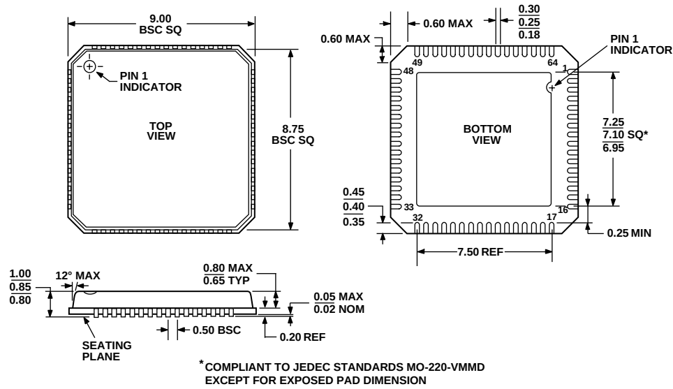
Figure 42. 64-Lead Lead Frame Chip Scale Package [LFCSP] 9 mm x 9 mm Body (CP-64-3)
