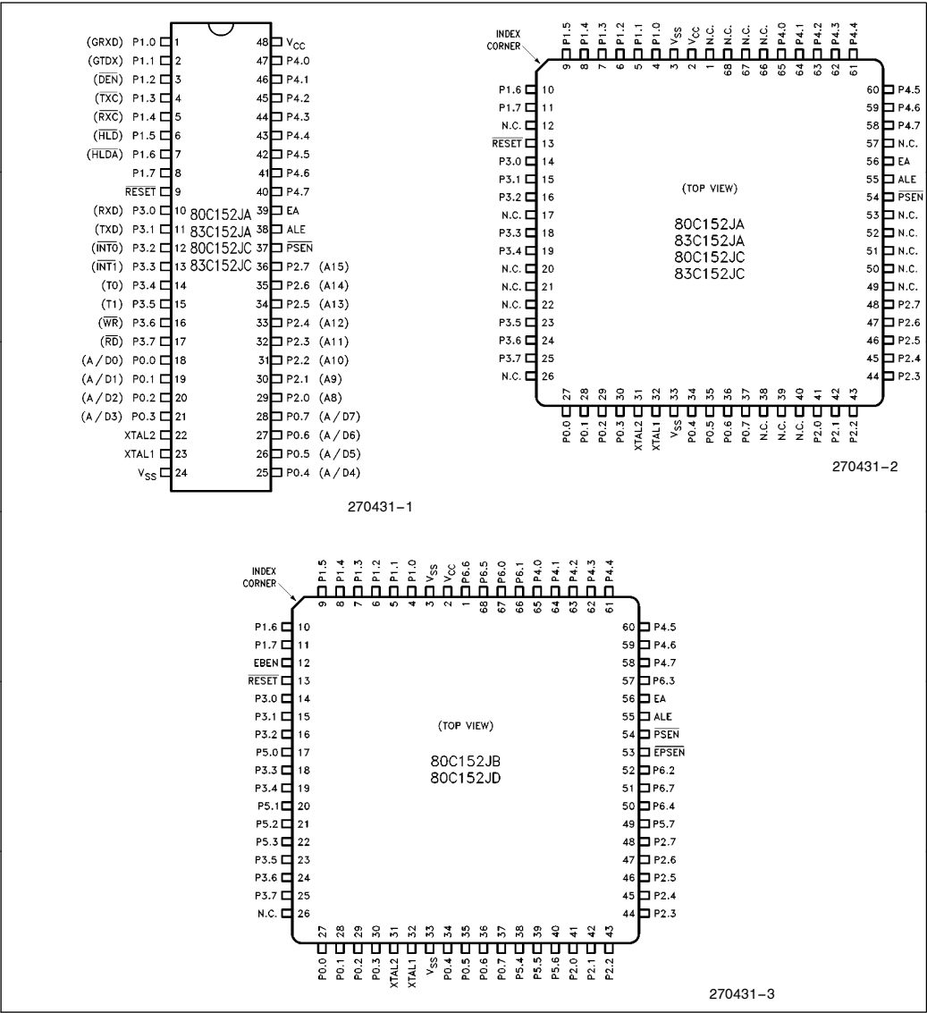
Figure 1. Connection Diagrams
