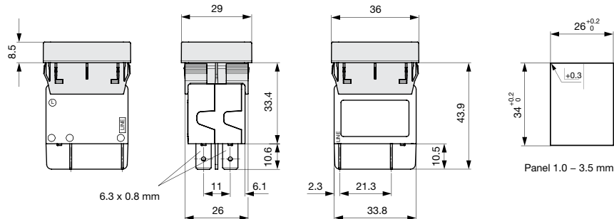
Accessories / CZM25, factory mounted transparent cover, antibacterial, IP65
