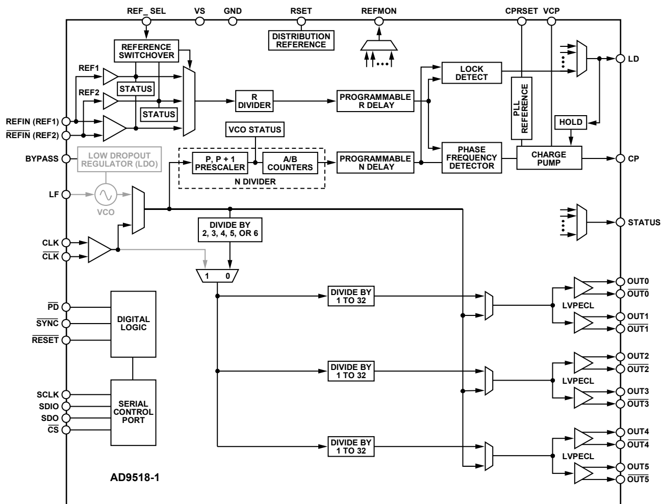
Figure 28. High Frequency Clock Distribution or External VCO &gt; 1600 MHz
