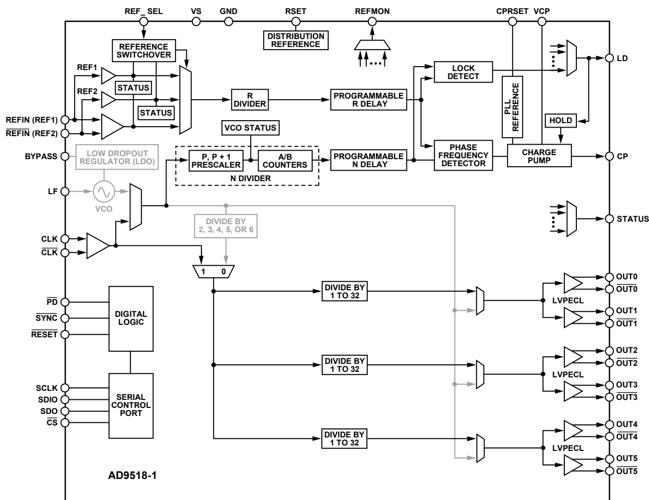
Figure 30. Clock Distribution or External VCO \leq 1600 MHz
