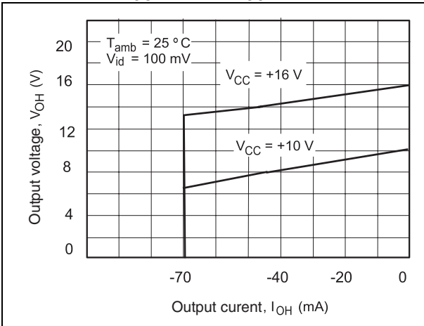
Figure 6. High level output voltage vs. high level output current ( V_{CC} = +16 V , V_{CC} = +10 V )
