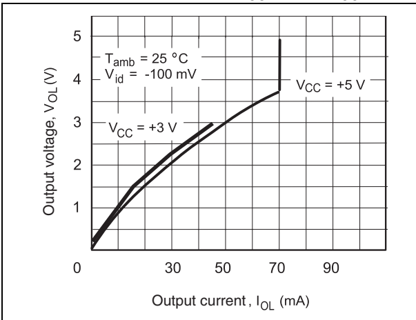
Figure 4. Low level output voltage vs. low level output current ( V_{CC} = +5 V , V_{CC} = +3 V )
