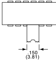
EXTENDED SIDE ACTUATOR
