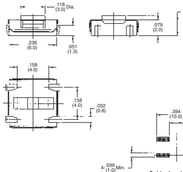
Solder Land Dimension
