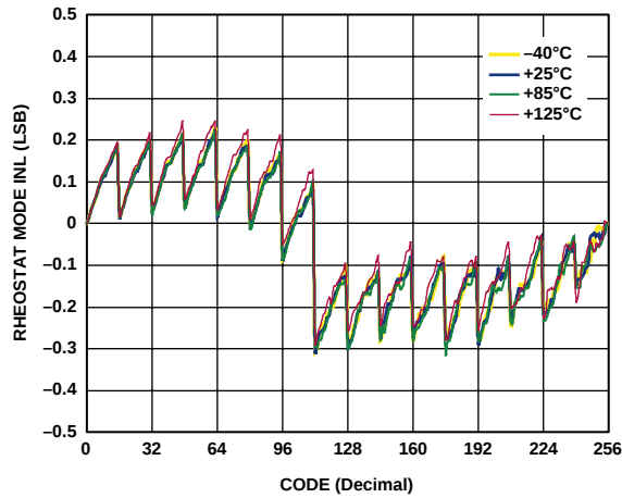
Figure 11. R-INL vs. Code vs. Temperature, V_{DD} = 5\text{ V}
