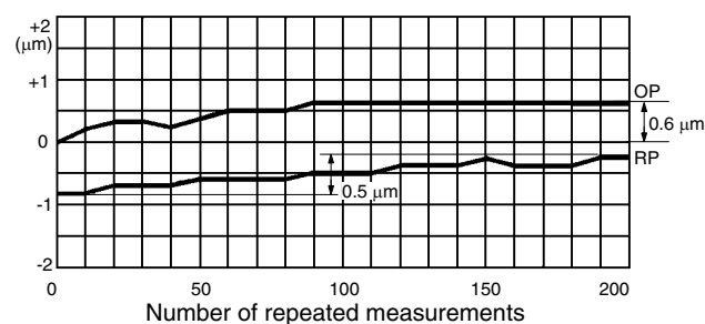
Slim Type (Solid-state Output) With Repeat Accuracy of 1 \mu\text{m} max. D5A-5□□□ Series
