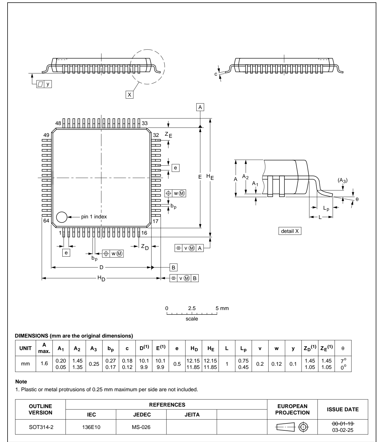
Fig 51. Package outline LQFP64 (SOT314-2)
