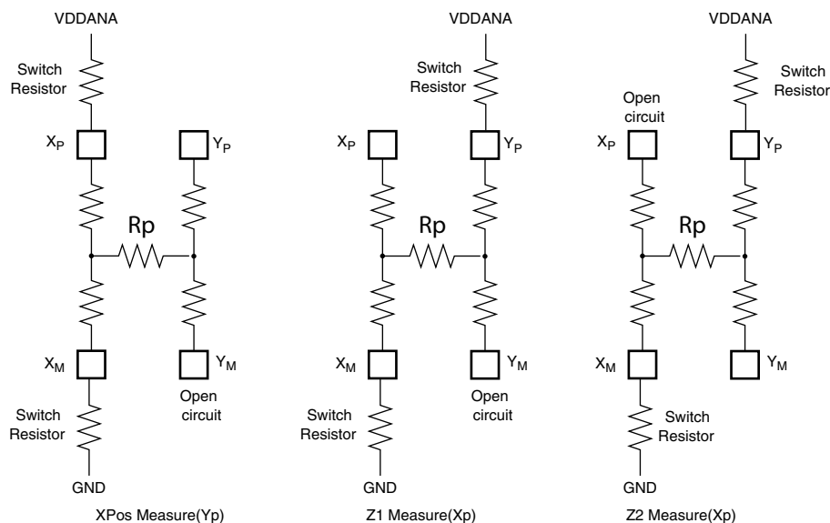
Figure 42-7. Pressure Measurement
