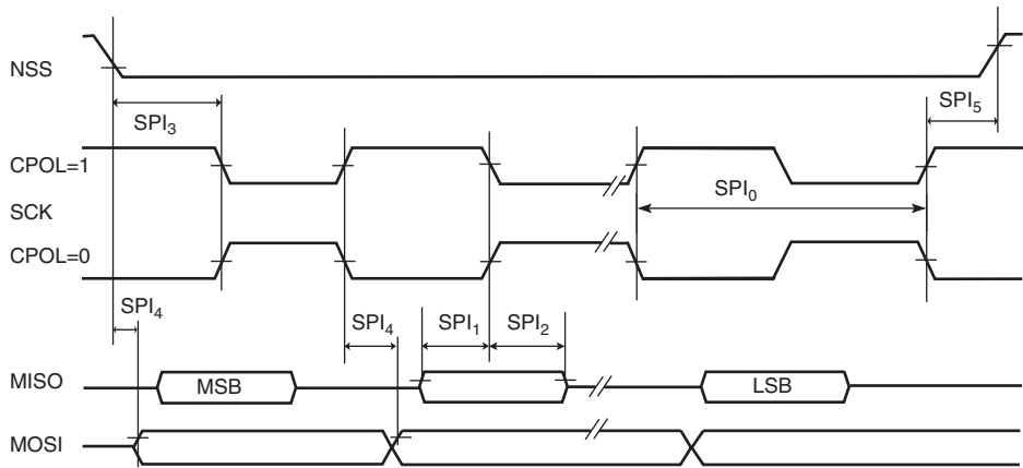
Figure 47-26.USART SPI Master Mode
