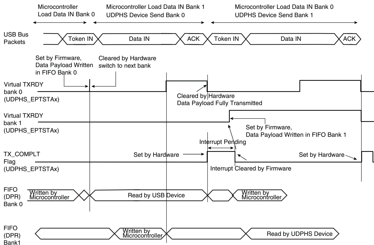
Figure 32-10.Data IN Transfer for Endpoint with Two Banks
