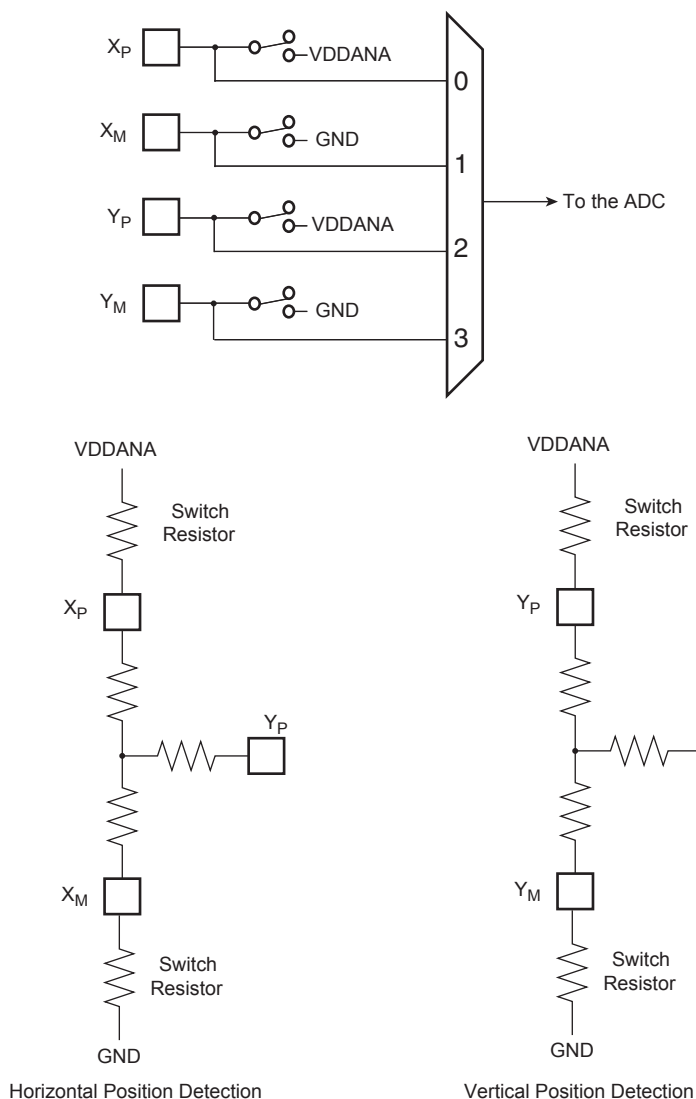
Figure 42-6. Touchscreen Switches Implementation
