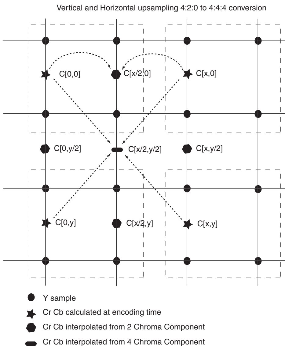
Figure 46-2. 4:2:2 Upsampling Algorithm
