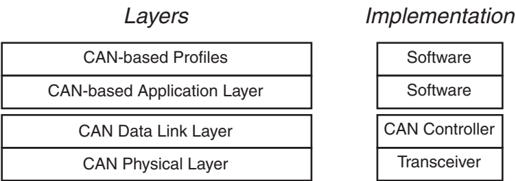
Figure 41-2. Application Block Diagram
