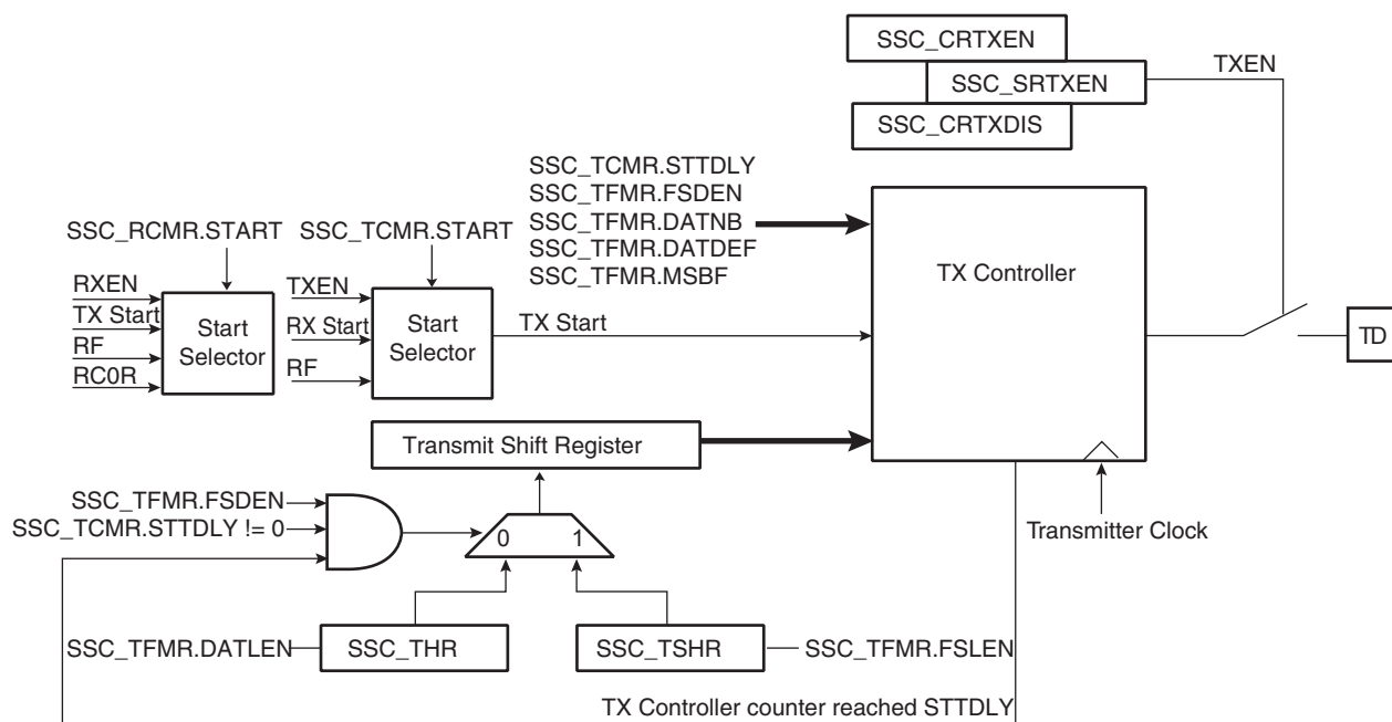
Figure 44-8. Transmitter Block Diagram
