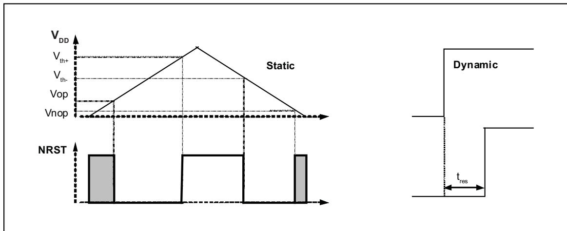
Figure 47-5. General Presentation of POR Behavior
