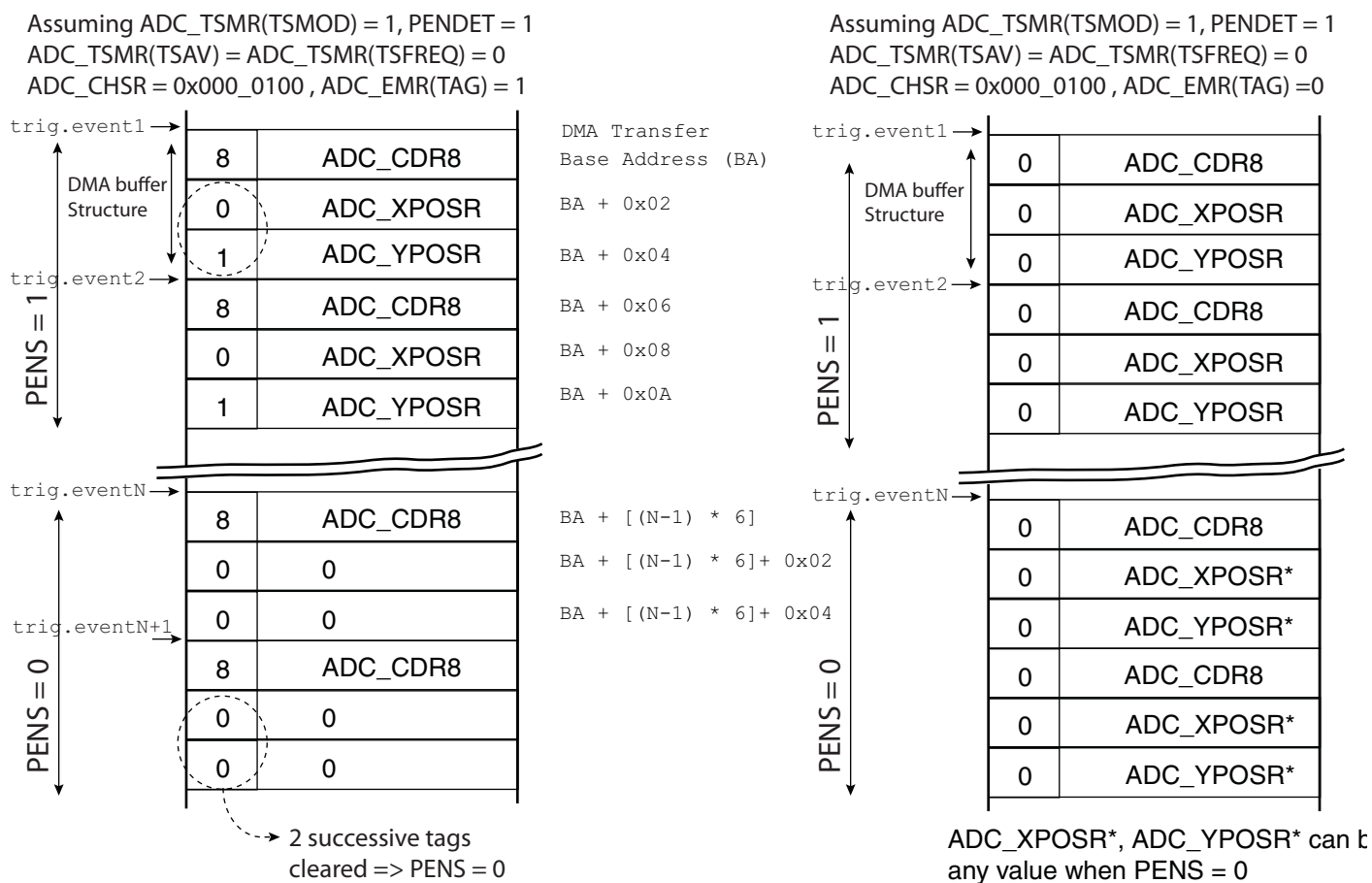
Figure 42-15. Buffer Structure with and without pen detection enabled
