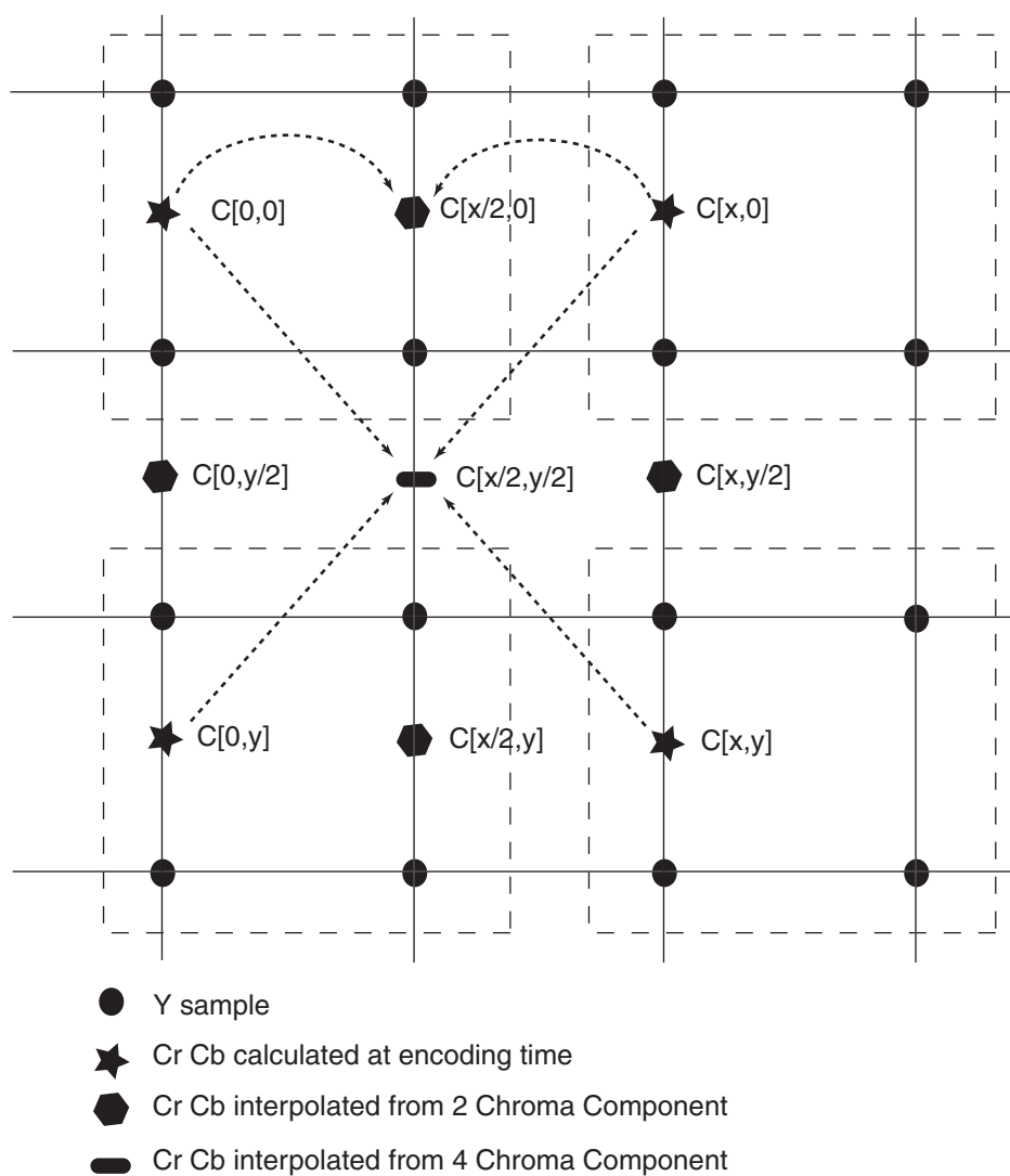
Figure 46-5. 4:2:0 Upsampling Algorithm
