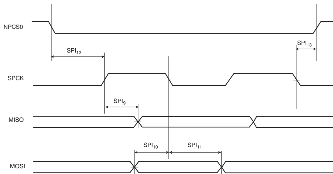
Figure 47-12.SPI Slave mode 1 and 2
