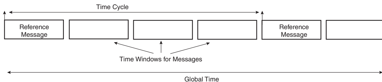
Figure 41-20. Time Triggered Principle
