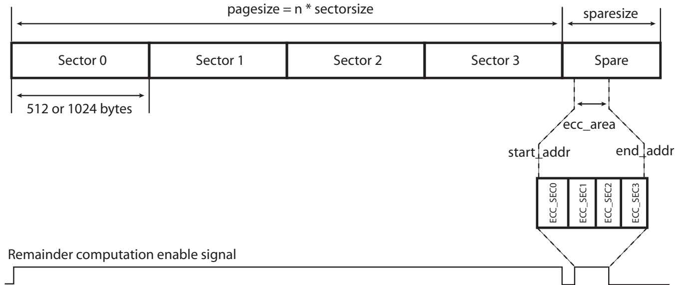
Figure 27-6. Read Operation
