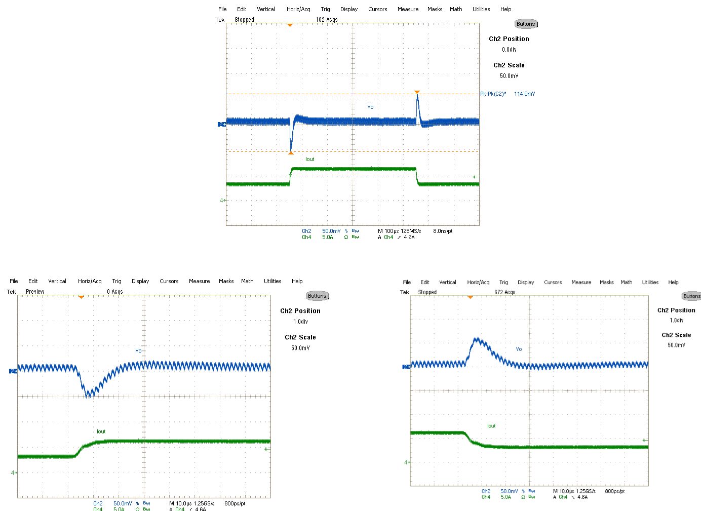
Fig. 13. Transient Response, 3A to 6A step 2.5A/\mu s Ch_2: V_o , Ch_4: I_o
