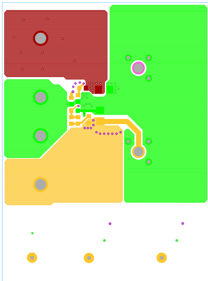
FIGURE 5. BOTTOM LAYER ETCH
