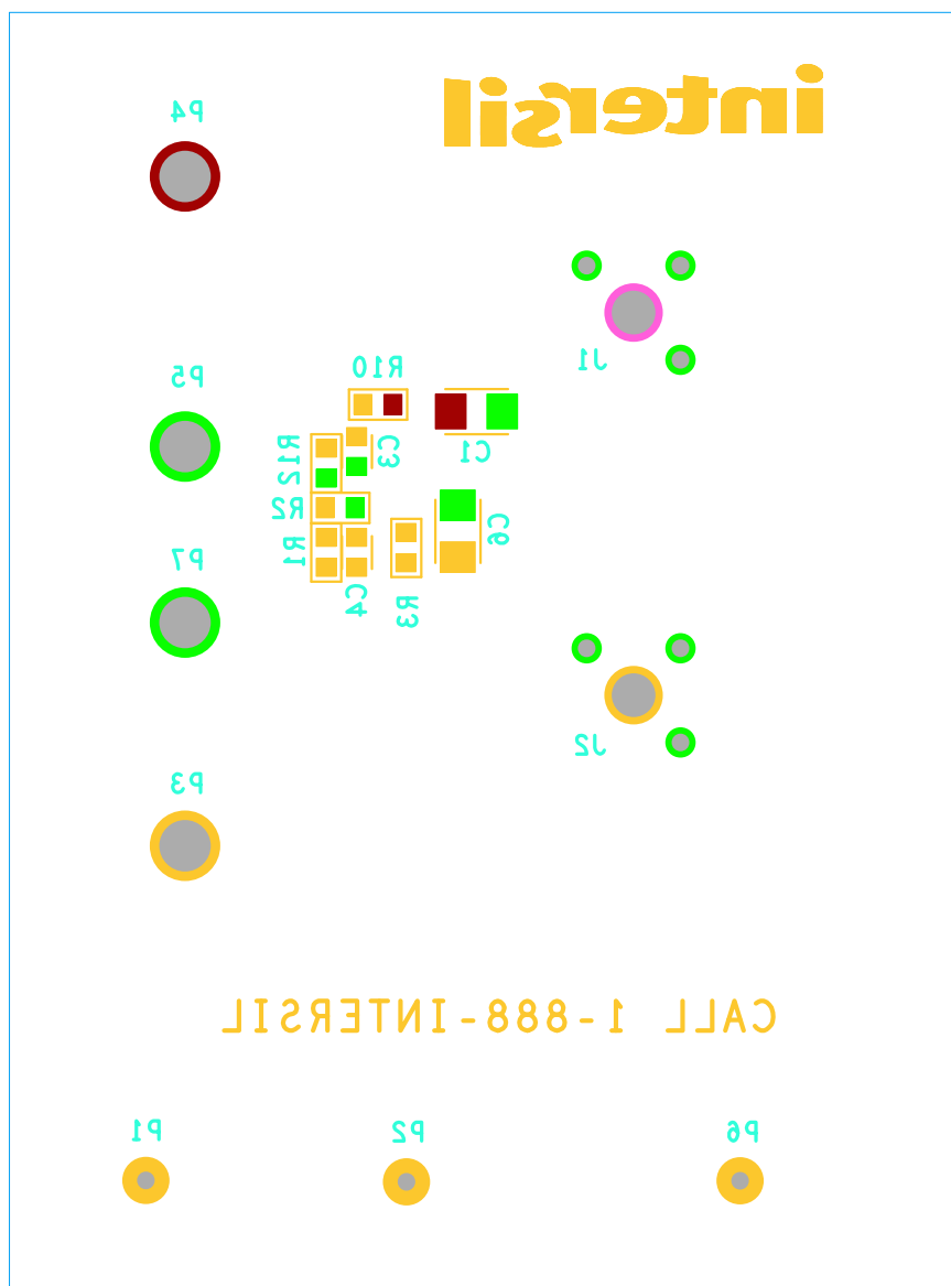
FIGURE 6. BOTTOM LAYER COMPONENTS
