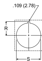
Panel Cutout
