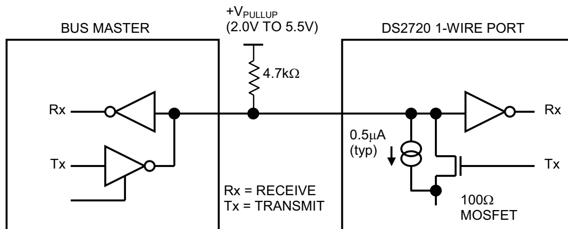
Figure 10. 1-WIRE BUS INTERFACE CIRCUITRY
