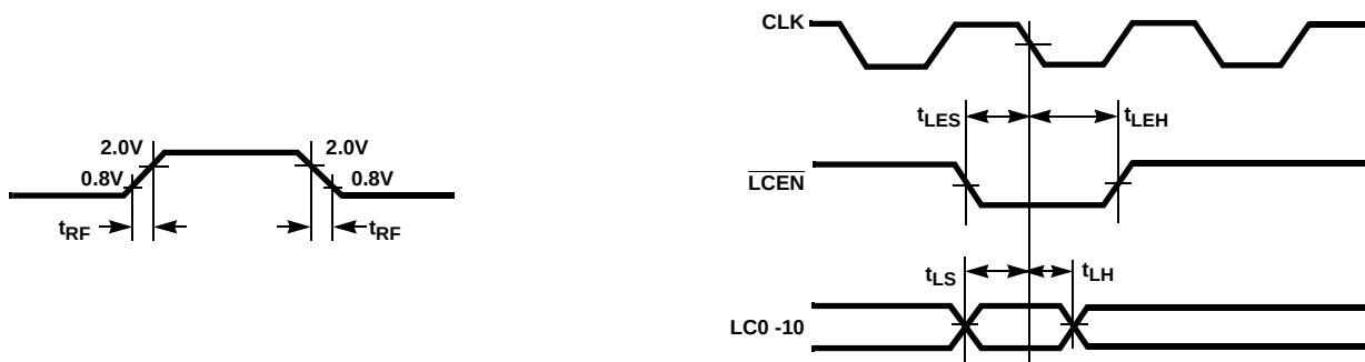
FIGURE 3. OUTPUT RISE AND FALL TIMES
